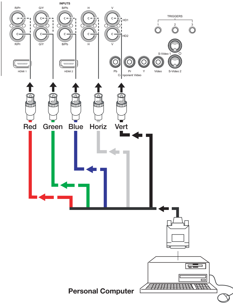
Figure 3-12. Analog RGB Connections
